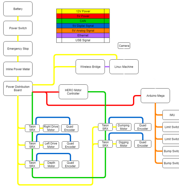
Figure 12: IBox Electrical Diagram
